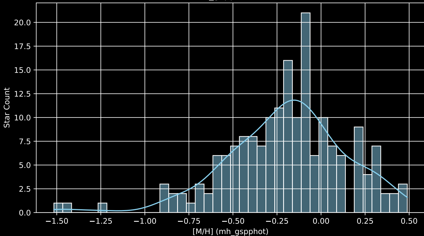
APOGEE DR17 Field: [265-33-O_TESS [M/H] (mh_gspphot) (n= 182)
