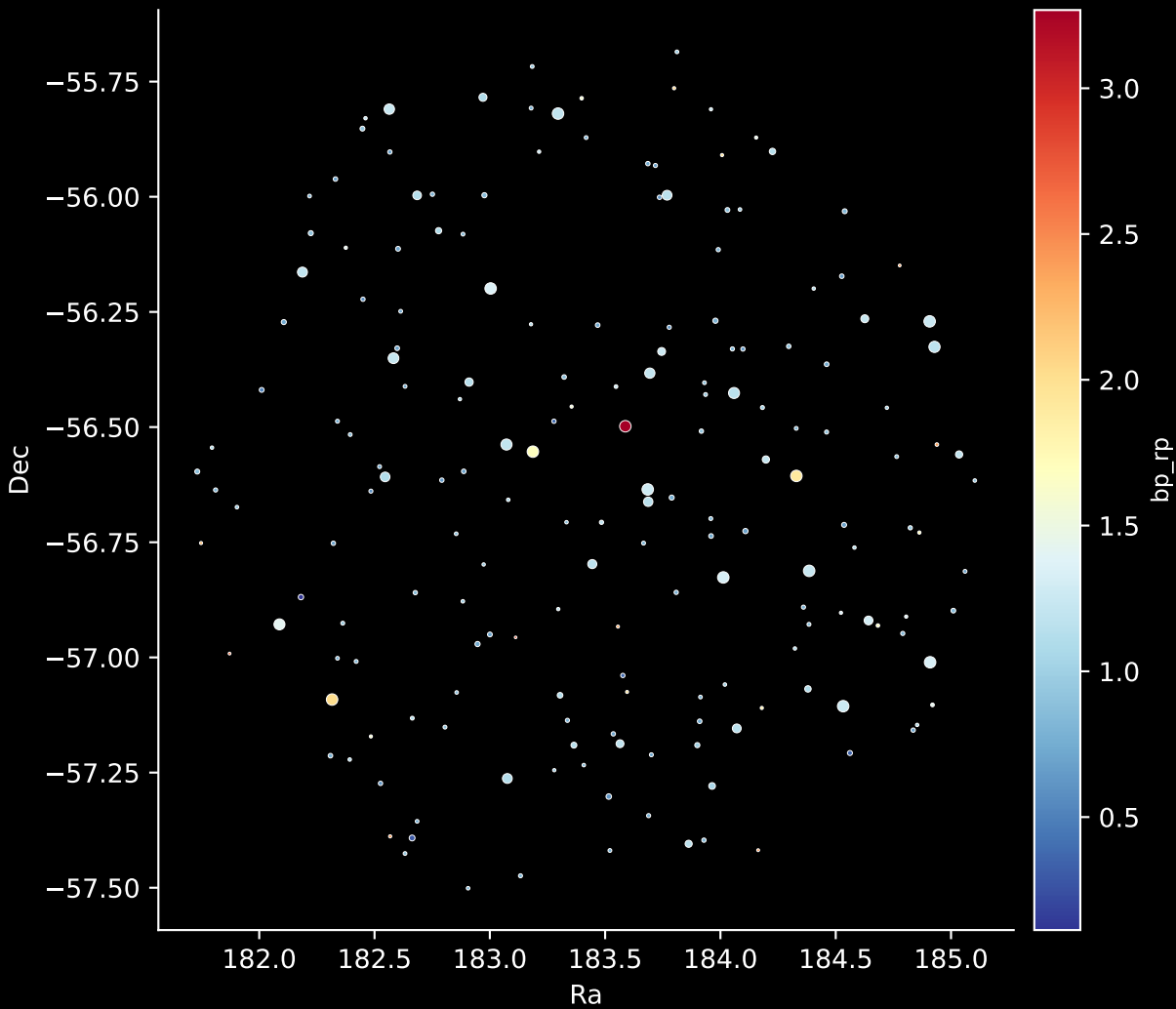
APOGEE DR17 Field: [265-33-O_TESS] Stars: 184
