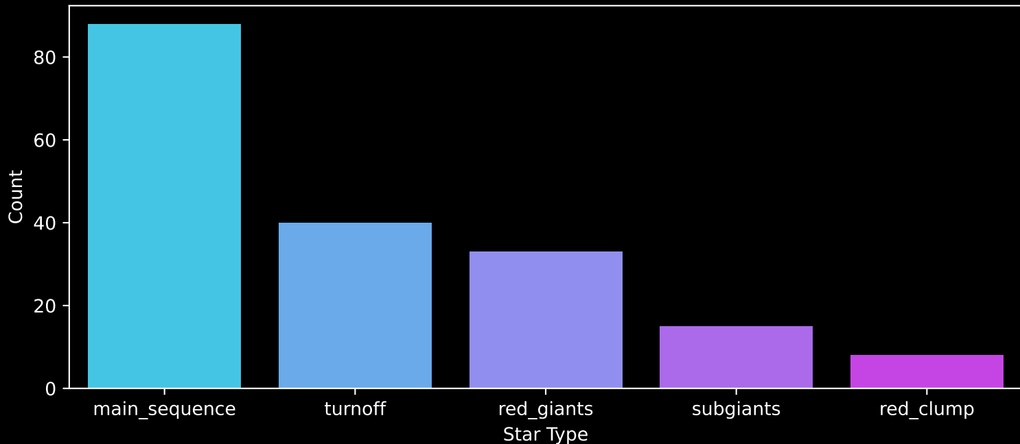
APOGEE DR17 Field: [265-33-O_TESS] Count plot of Star Type
